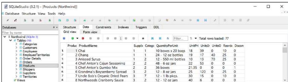
Figure 10.5: The Data tab showing the rows in the Products table
