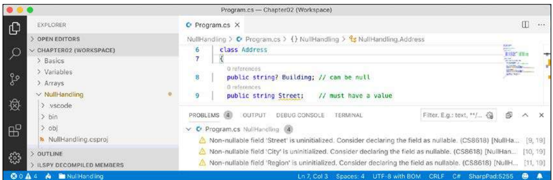
Figure 6.2: Warning messages about non-nullable fields in the PROBLEMS window
